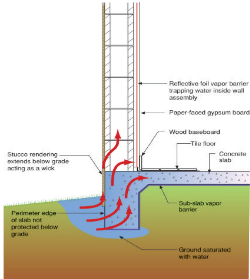
Figure 1 Slab-on-grade floor detail (illustration courtesy of Dr. Joseph Lstiburek, Building Science Corp.)
